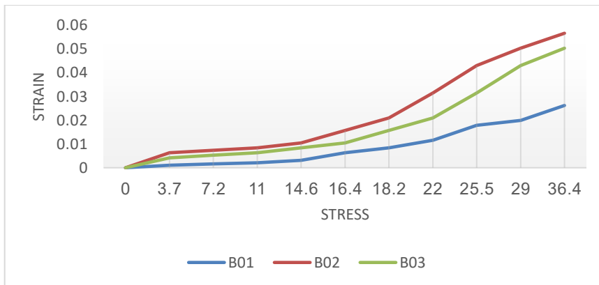
Figure 13. Stress vs. strain (simulation)
