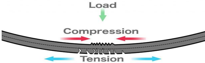
Figure 2. Tensile and compressive stresses
