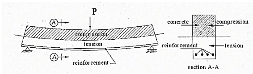
Figure 4. The bending stress (Ft).
